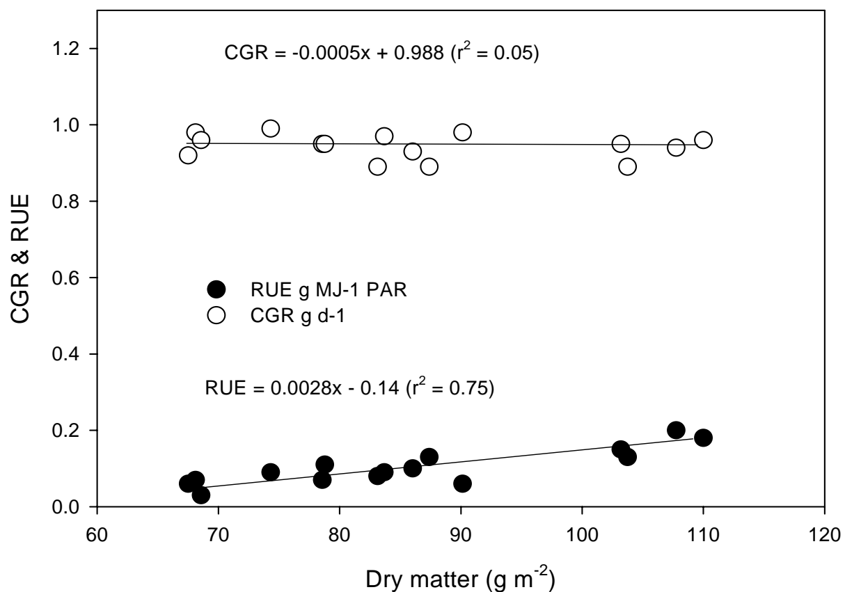
Fig. 2. Crop growth rate (g d -1 ) and radiation use efficiency (g DM MJ -1 PAR absorbed ) in relation to dry matter production of different alfalfa lines in Peshawar.
