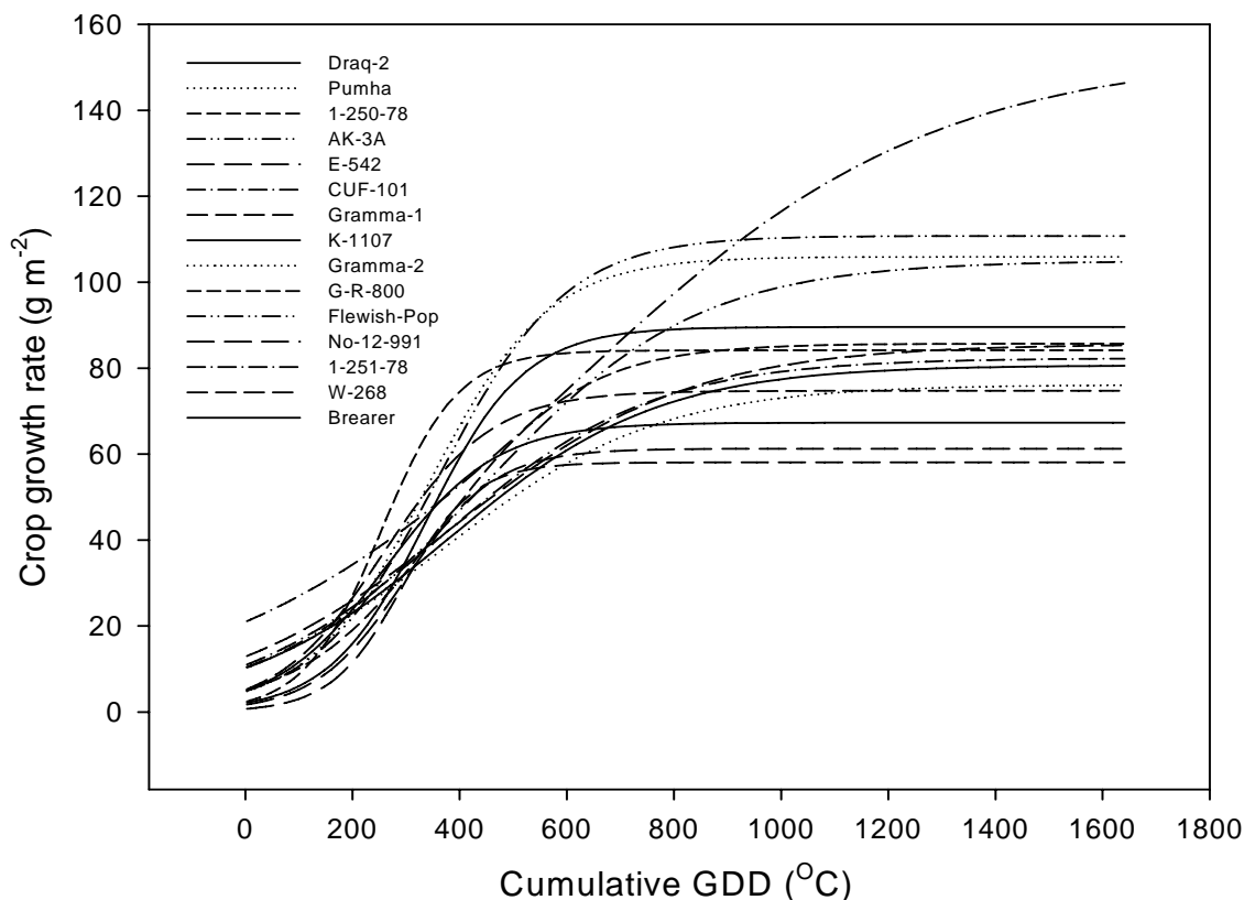
Fig. 1. Crop dry matter ( \text{g m}^{-2} ) in relation to cumulative growing degree days ( ^{\circ}\text{C} ) of the different alfalfa lines in early summer in Peshawar.
