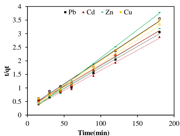
Fig. 7. Linear expression of PSO kinetics of biosorption for cadmium, copper, lead, and zinc ions. (Contact time = 60 min for cadmium, copper, lead ions and 45 min for zinc, pH=5.0 for Pb & Cd ions and 6.0 for zinc & copper ions, biomass dose= 1 gL -1 ). Dotted lines show the PSO data of WB and solid lines show that of BWE.
