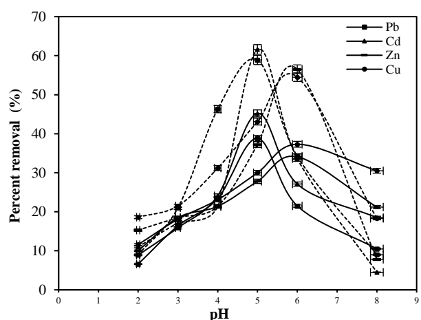
Fig. 4. Effect of pH on percent removal of WB (dotted lines) and BWE (solid lines) for cadmium, copper, lead, and zinc. ( C_o= 20 \text{ mgL}^{-1} , Contact time = 60 min for Cd, Cu, Pb ions and 45 min for Zinc ions, biomass dose= 1 gL -1 ).
