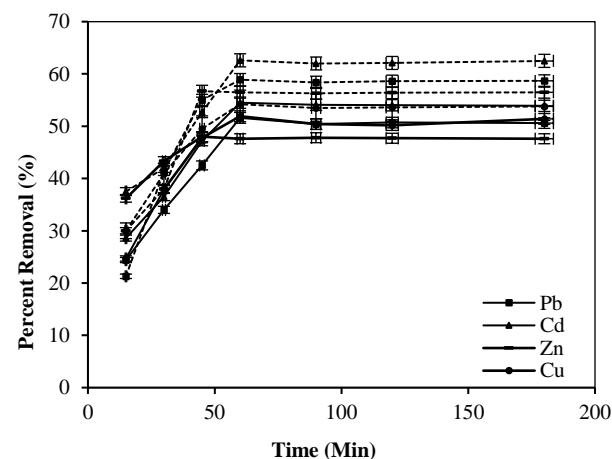
Fig. 5. Effect of contact time on biosorption studies of WB (dotted lines) and BWE (solid lines) for cadmium, copper, lead, and zinc ions. ( C_o= 20 \text{ mgL}^{-1} , pH=5.0 for Pb & Cd ions and 6.0 for Zn & Cu ions, biomass dose= 1 gL -1 ).
