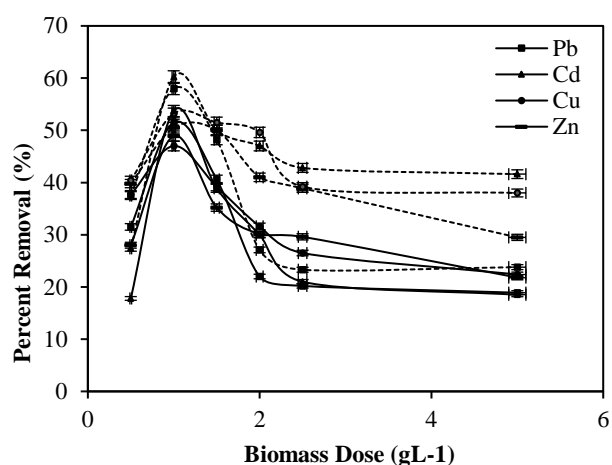
Fig. 3. Effect of amount biomass dosage on percent removal of Cadmium, Copper, Lead, and Zinc. The dotted lines represent the WB and the solid line present the BWE ( C_o= 20 \text{ mgL}^{-1} , pH=5.0 for Lead, Cadmium and 6.0 for Copper and Zinc. Time of contact = 60 min for Cadmium, Copper, Lead, and 45 min for zinc).
