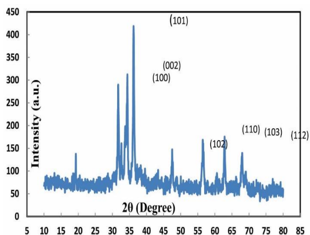
Fig. 3 D. XRD pattern indicating the presence of ZnONPs peaks
