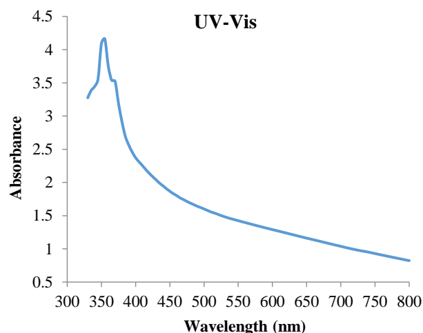
Fig. 1. Absorption spectrum of ZnONPs showing a sharp peak at 355nm wavelength.
