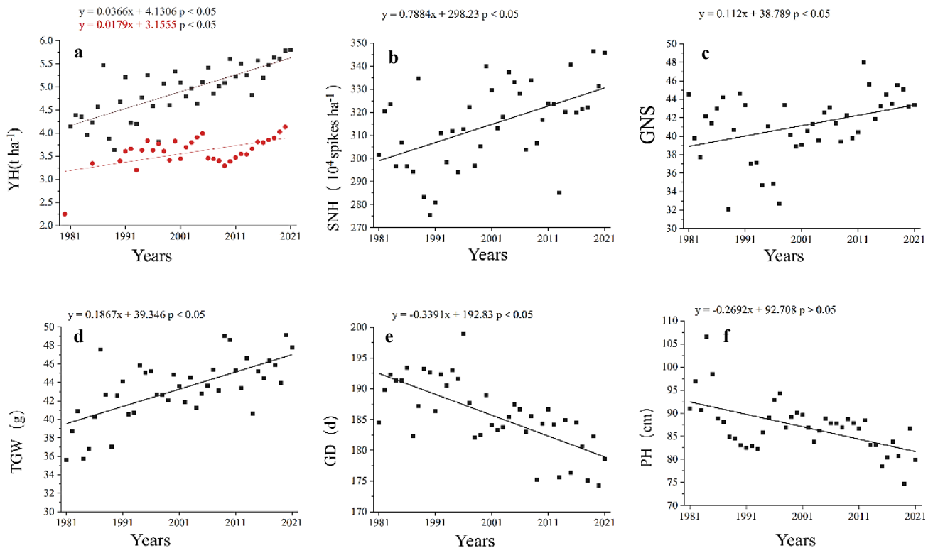
Fig. 3. The average value of yield and yield components of wheat lines in regional test from 1981–2021. a The yield per hectare (YH) of regional test and actual yield in Sichuan Province from 1981–2021. Black for regional test, red for actual yield in Sichuan Province. b The spikes number per hectare (SNH) of regional test from 1981–2021. c The grain number per spike (GNS) of regional test from 1981–2021. d The thousand grain weight (TGW) of regional test from 1981–2021. e The growth duration (GD) of regional test from 1981–2021. f The plant height (PH) of regional test from 1981–2021.
