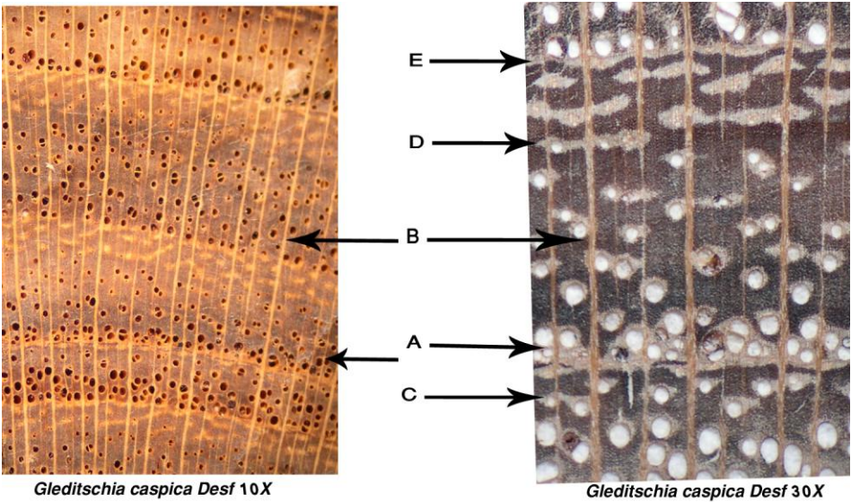
Fig. 13. Cross section of Caspian Locust ( Gleditschia caspica ), Ring – porous wood. (A) Earlywood, tyloses absent (B) Rays are variable in size, the largest conspicuous to the eye (C) Aliform parenchyma (D) Aliform confluent parenchyma (E) Aliform confluent parenchyma in outer in last part of latewood.
