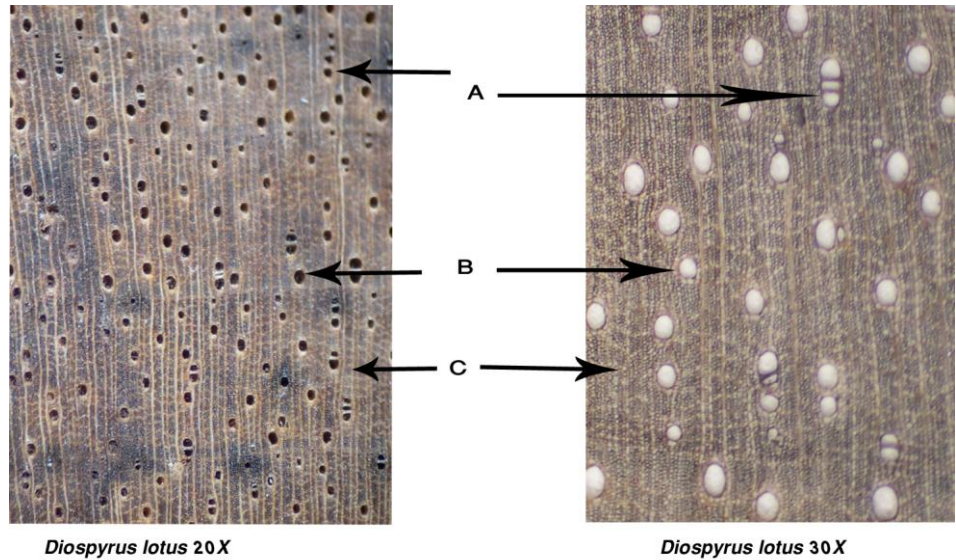
Fig. 5. Cross section of Persimmon ( Diospyros lotus ), Diffuse – porous wood. (A) Pores solitary or in radial multiples (2-3) and with thick-walled (B) Vasicentric parenchyma which is visible with high magnification in chalky surface (C) Rays fine, visible with lines.
