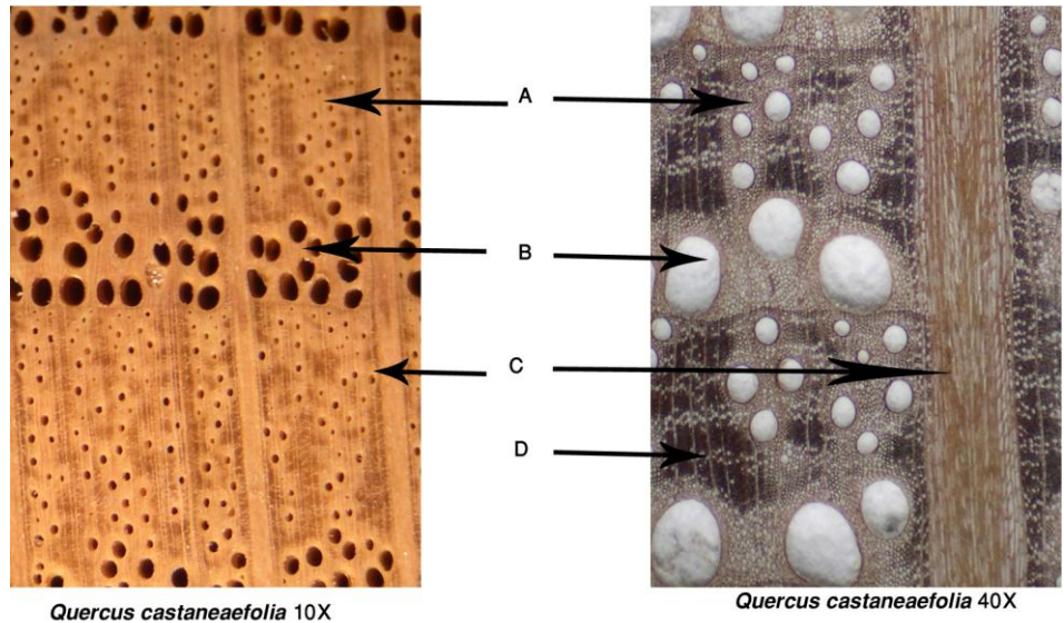
Fig. 12. Cross section of Oak ( Quercus castaneaefolia ), Ring – porous wood. (A) Latewood vessels which are exclusively solitary and flame like, surrounded with lighter tissue which is axial parenchyma (B) Earlywood vessel which is surrounded with lighter tissue which is vasicentric tracheid and axial parenchyma (C) Wide rays which is easily visible without lens (D) Axial parenchyma in tangential bands.
