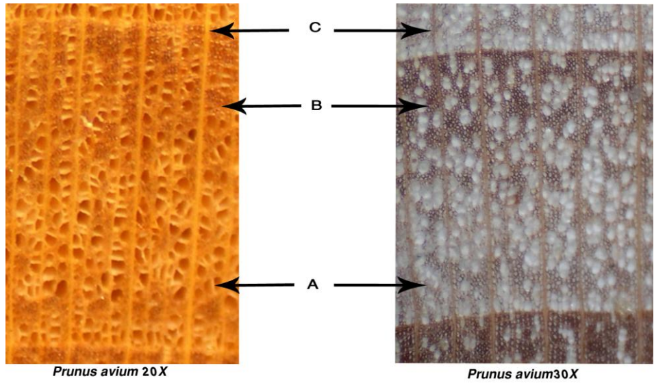
Fig. 7. Cross section of Wild cherry ( Prunus avium ), Diffuse – porous wood. (A) Fairly large vessels have been gathered along initial early wood and quantity of vessels get much more lower in latewood, pores are clusters and multiple (2-5) (B) The number of vessels in latewood lower than earlywood (C) Rays are visible without lens.
