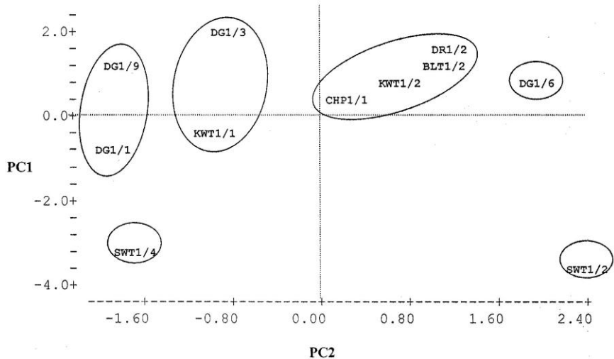
Fig. 1. Plot of principal component 1 and 2 for different accessions of Lasiurus scindicus .
