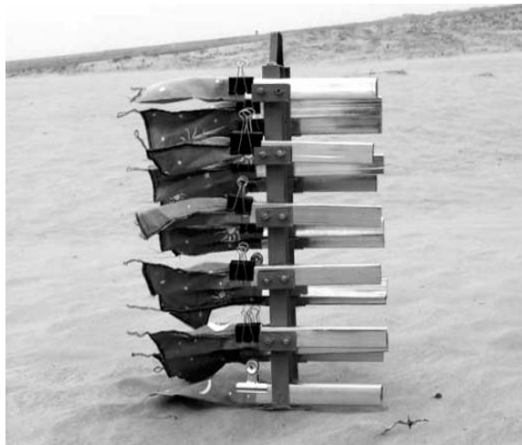
Fig. 2. Sand collection instrument.
