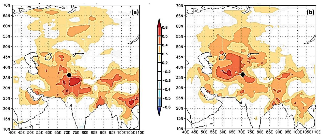
Fig. 5. Spatial correlation of growing season (a) winter (pDec-Feb) (b) spring (Mar-May) mean precipitation with the TRW chronology for the period 1967–2021. The sample site is shown by the black spot.
