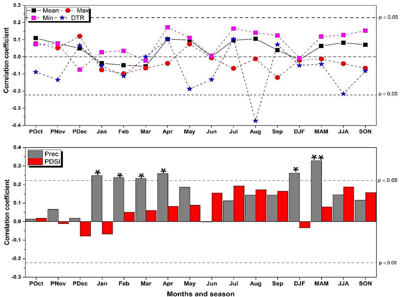
Fig. 4. The upper panel of the figure illustrates the correlation between the Dir Upper chronology and various temperature variables (Tmax, Tmean, Tmin, and DTR). The lower panel represents the relationship between the DU chronology and precipitation, as well as the Palmer Drought Severity Index (PDSI), spanning from October of the previous year to September of the current year. The analysis incorporates seasonal data from the Dir weather station, covering the period from 1967 to 2021. The horizontal dashed line and single asterisk (*) indicate significance at p < 0.05 , while the double asterisk (**) denotes significance at p < 0.01 .
