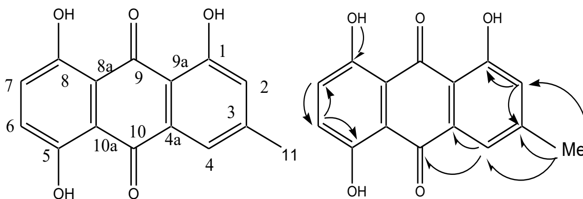
Fig. 2. Positions of carbons and key HMBC correlations of compound 2. H→C.
