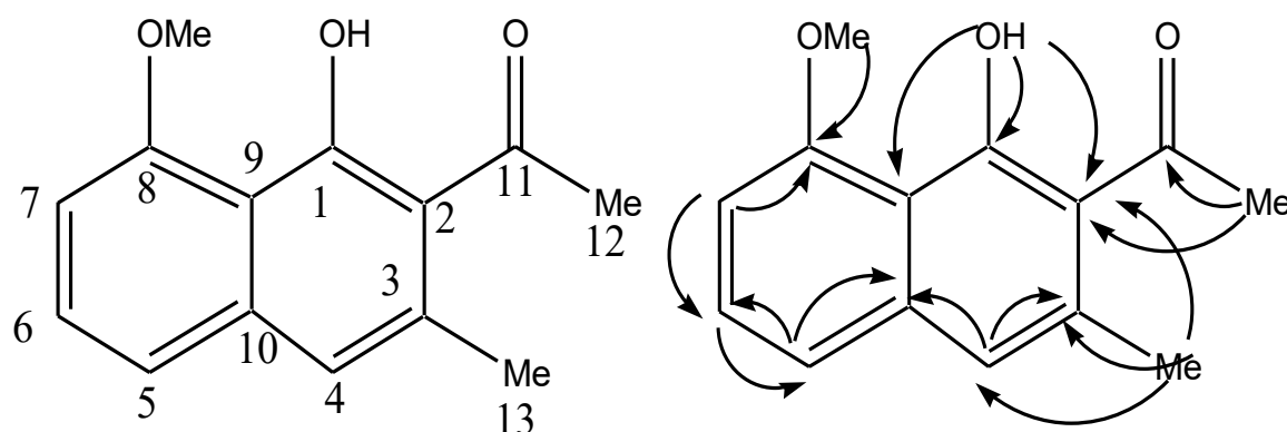
Fig. 1. Positions of carbons and key HMBC correlations of compound 1. H→C.
