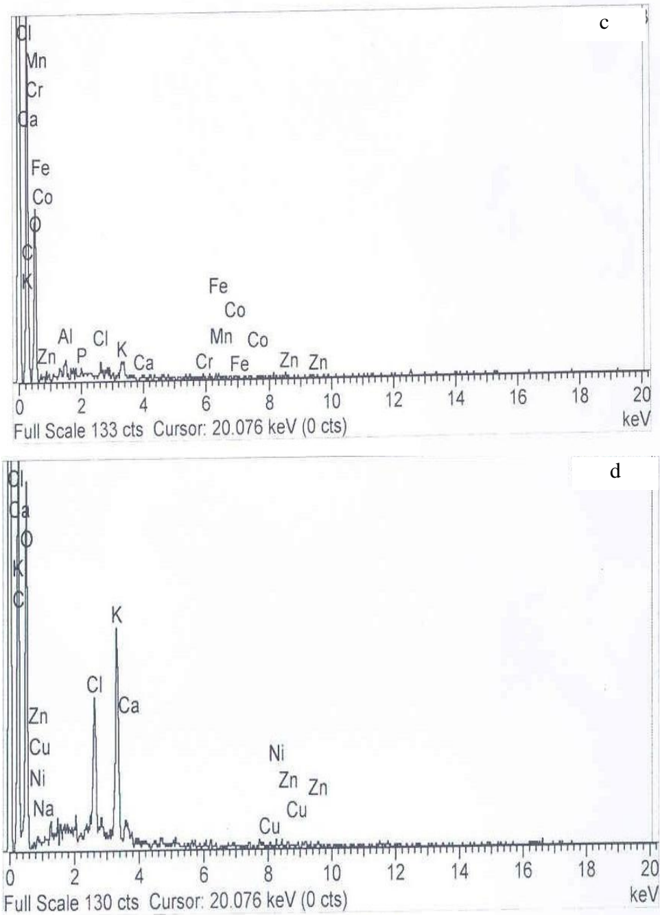
Fig. 1. Inorganic profile of the selected subfractions using SEM-EDX technique. Diverse nature of elements was recorded in the hexane (a), chloroform (b), butanol (c) and water (d) subfractions. Full scan of the subfraction was done to obtain complete informations.
