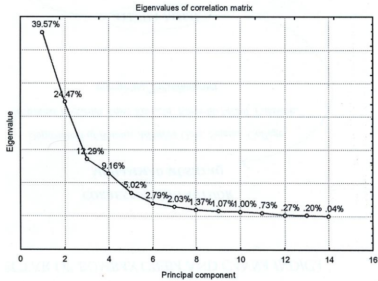
Fig. 2. Scree plot constructed for 14 principal components
