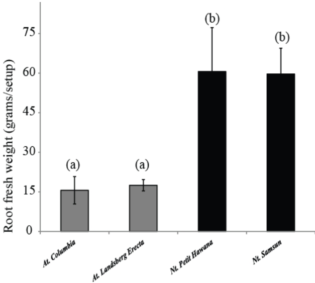
Fig. 3. Root fresh weight from Arabidopsis thaliana (At) ecotype Columbia and landsberg erecta , Nicotiana tabacum (Nt) var Petit havana and Samsun was calculated. For this roots were harvested after ten weeks of seed germination. After removing the extra medium (using a salad spinner), root fresh weigh was calculated in grams per setup. The bars represent standard deviation and letters indicated mean values that are significantly different (one way ANOVA; p < 0.05 ).
