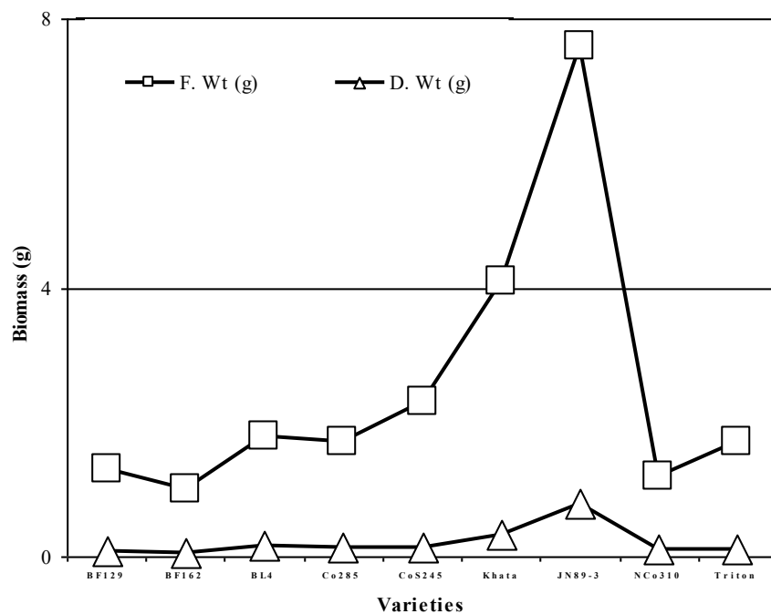
Fig. 4. Varietal response of sugarcane cultures to in vitro preservation for 3 months.
