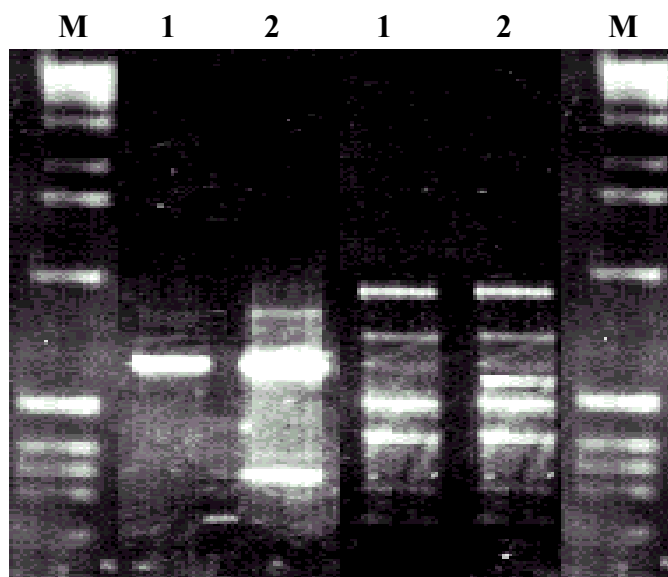
Fig. 2 Results of RAPD reactions involving two bulks (lane 1, salinity tolerant and lane 2 salinity sensitive) using 10-mer primers OPR-14 and OPZ-10.
