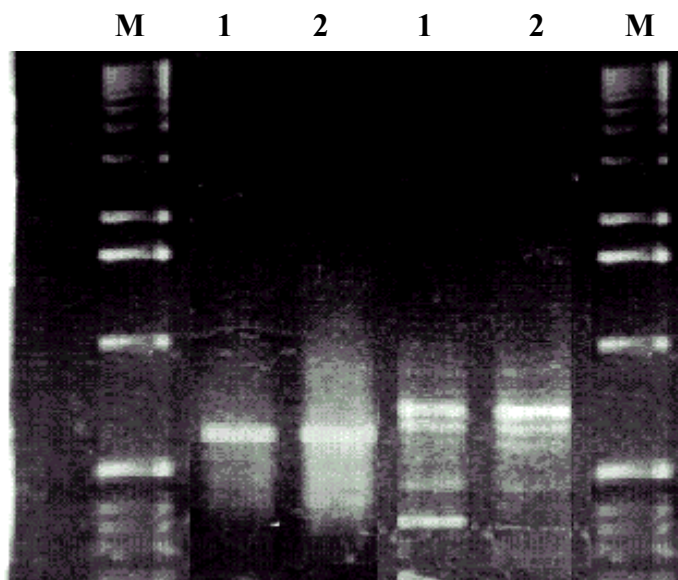
Fig. 1 Results of RAPD reactions involving two bulks (lane 1, salinity tolerant and lane 2 salinity sensitive) using 10-mer primers OPM-07 and OPM-14
